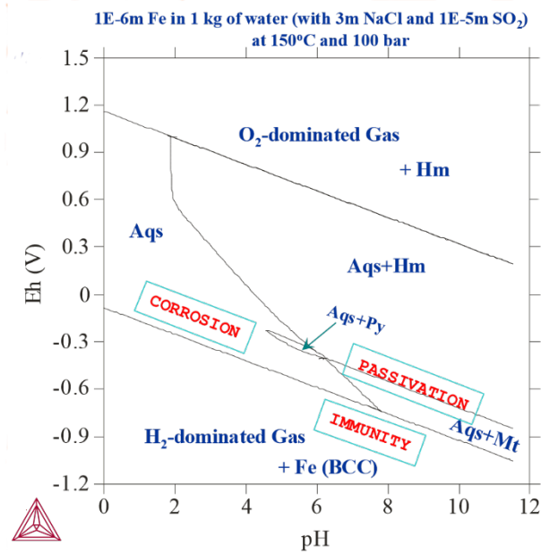
Figure 6: 1E-6 m Fe actively reacted with 1 kg of water, 3m NaCl and 1E-5 m SO 2 at 150° C and 100 bar. Here, changing the temperature and pressure affects the stability fields of various Fe-oxides/sulphides.
