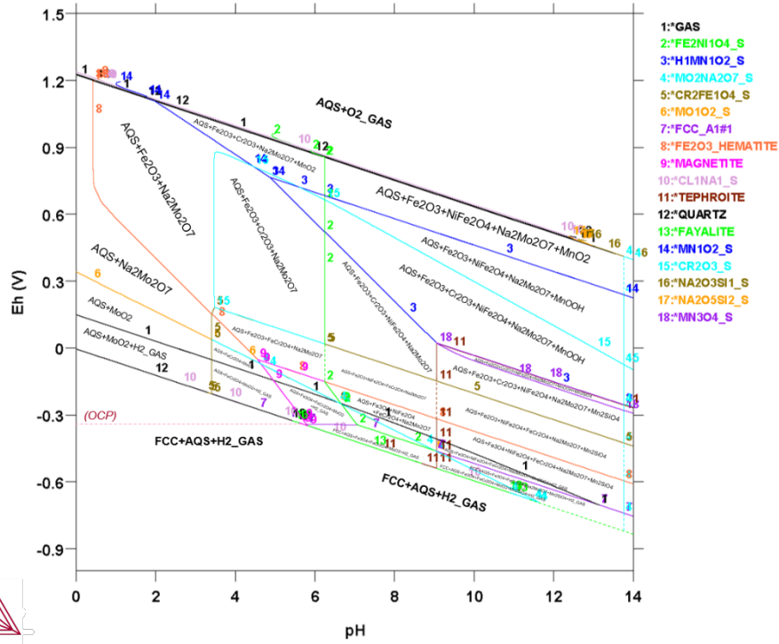
0.1m AISI4340 Steel in 0.6054m-NaCl Aqueous Solution, 25 C
