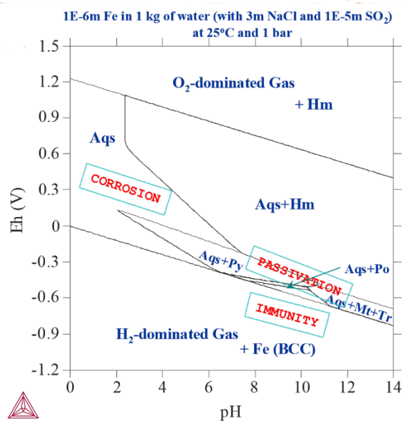
Figure 5: 1E-6 m Fe actively reacted with 1 kg of water, 3m NaCl and 1E-5 m SO 2 at 25° C and 1 bar. Introducing SO 2 into the system leads to the formation of various metal-sulphides (Py-pyrite, Popyrrhotite, Tr-troilite). In addition, the passivation region becomes larger.
