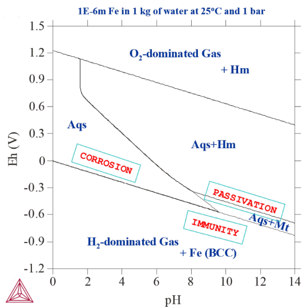
Figure 4: 1E-6 m Fe actively reacted with 1 kg of pure water at 25° C and 1 bar. Note that the active metal corrosion region gets enlarged as the initial Fe amount decreases from 1E-3m to 1E-6m.
