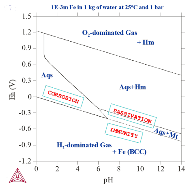
Figure 3: 1E-3 m Fe actively reacted with 1 kg of pure water at 25° C and 1 bar (as in the calculation in Pourbaix Diagrams with Gas Phase Included).
