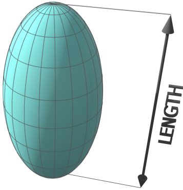
Figure 11: A prolate spheroid is a surface of revolution obtained by rotating an ellipse about its major axis.
