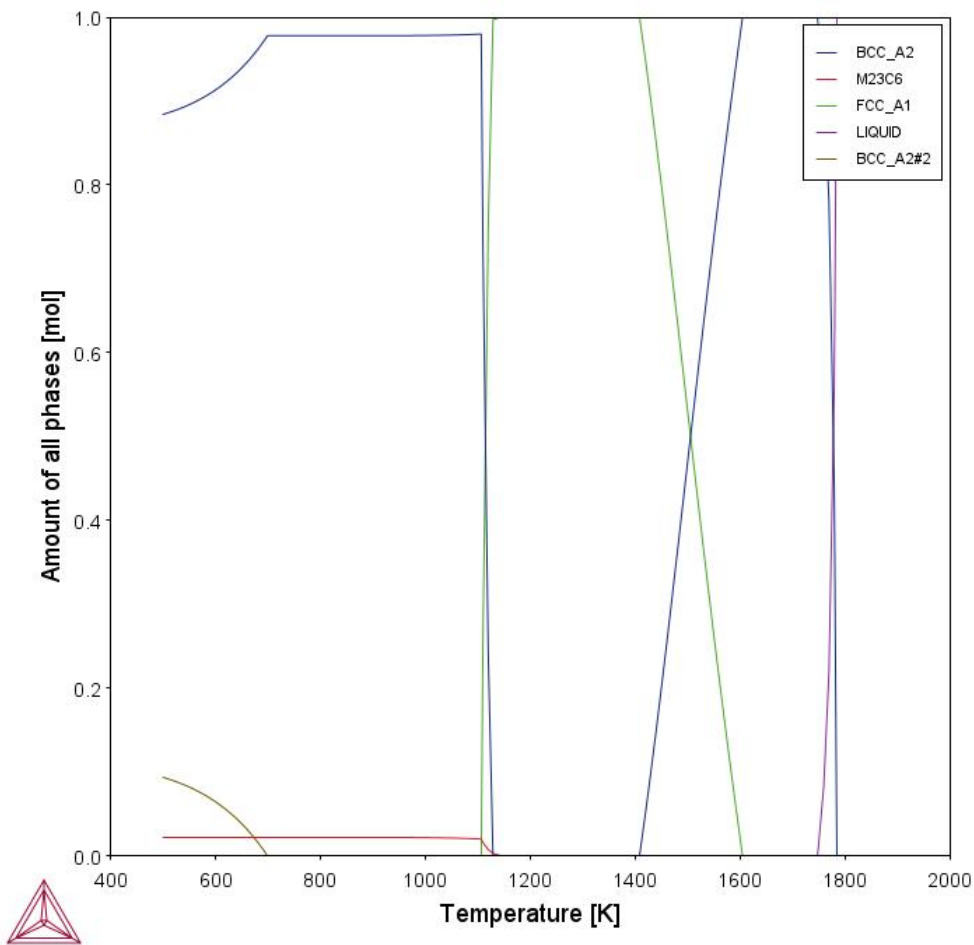
Figure 14: The Equilibrium Calculator and a one axis calculation is used to determine how the phases change with temperature.
