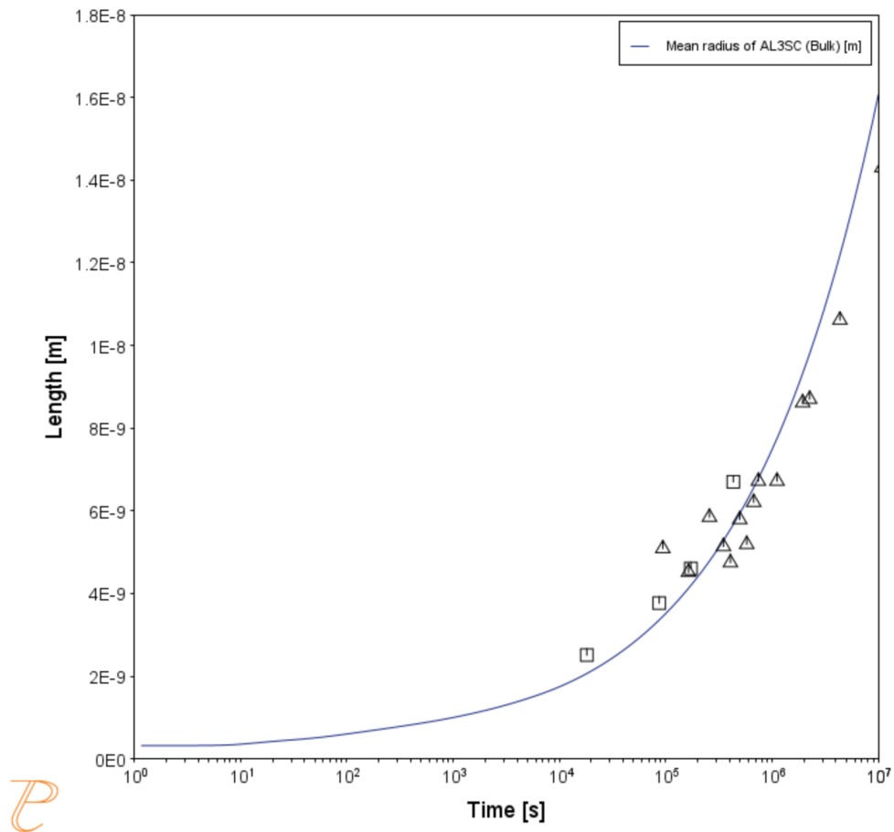
Figure 12: The mean radius of the AL3SC precipitate as a function of time.
