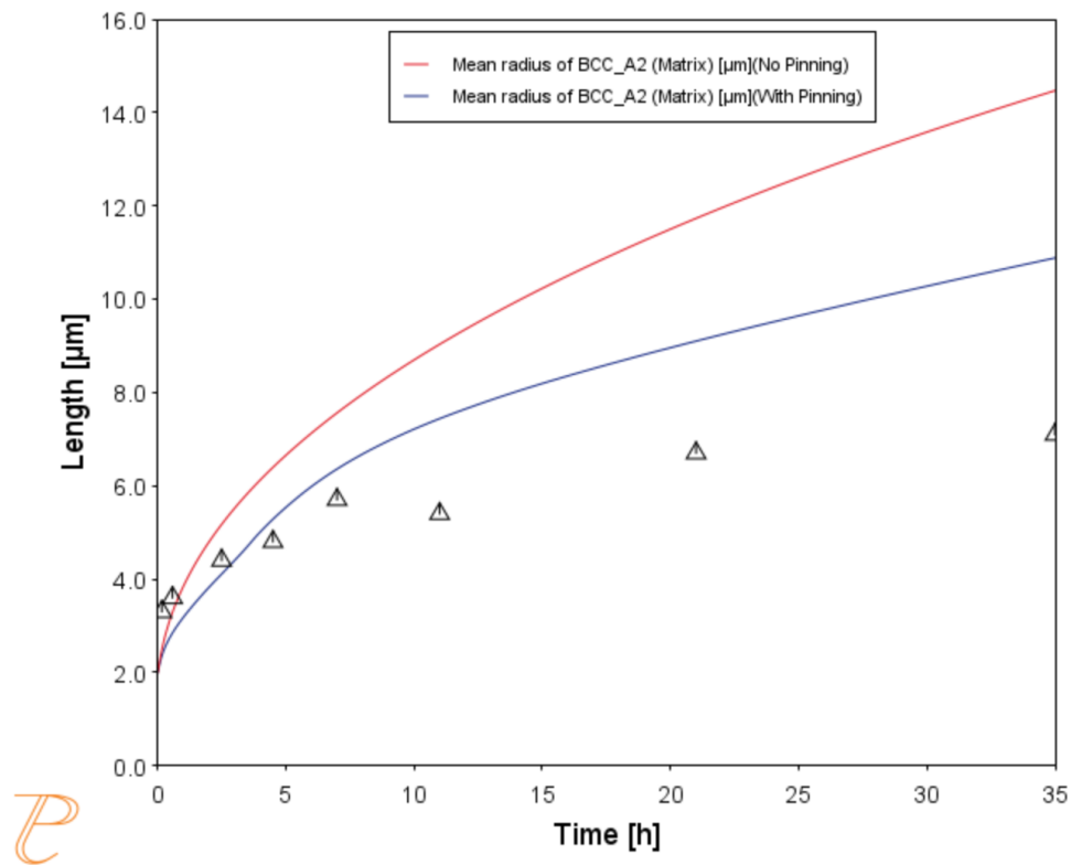
Figure 43: Result comparing the ferrite mean grain radius with and without pinning for the BCC-A2 phase and compared to experimental data [1975Hel].
