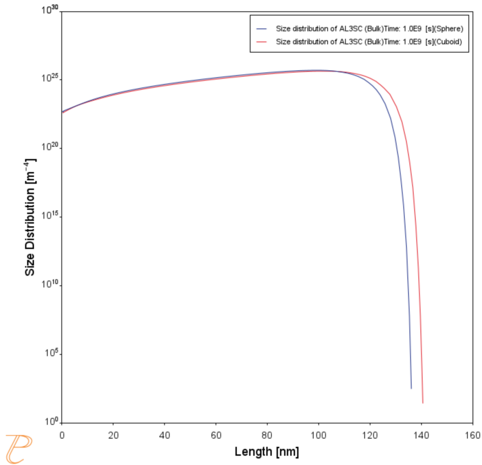
Figure 33: Particle size distribution (PSD).
