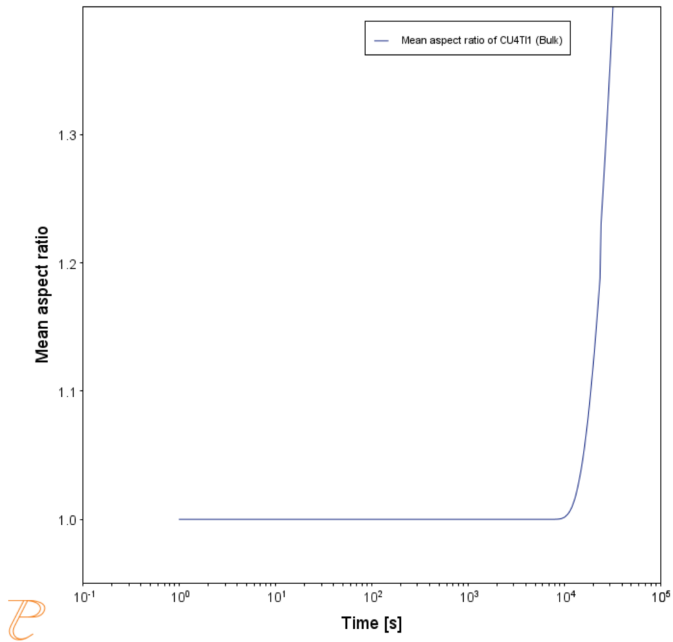
Figure 28: Mean Aspect Ratio.
