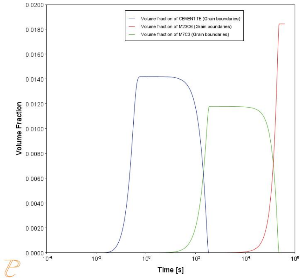
Figure 38: Volume fraction with no initial particle size distribution (PSD).
