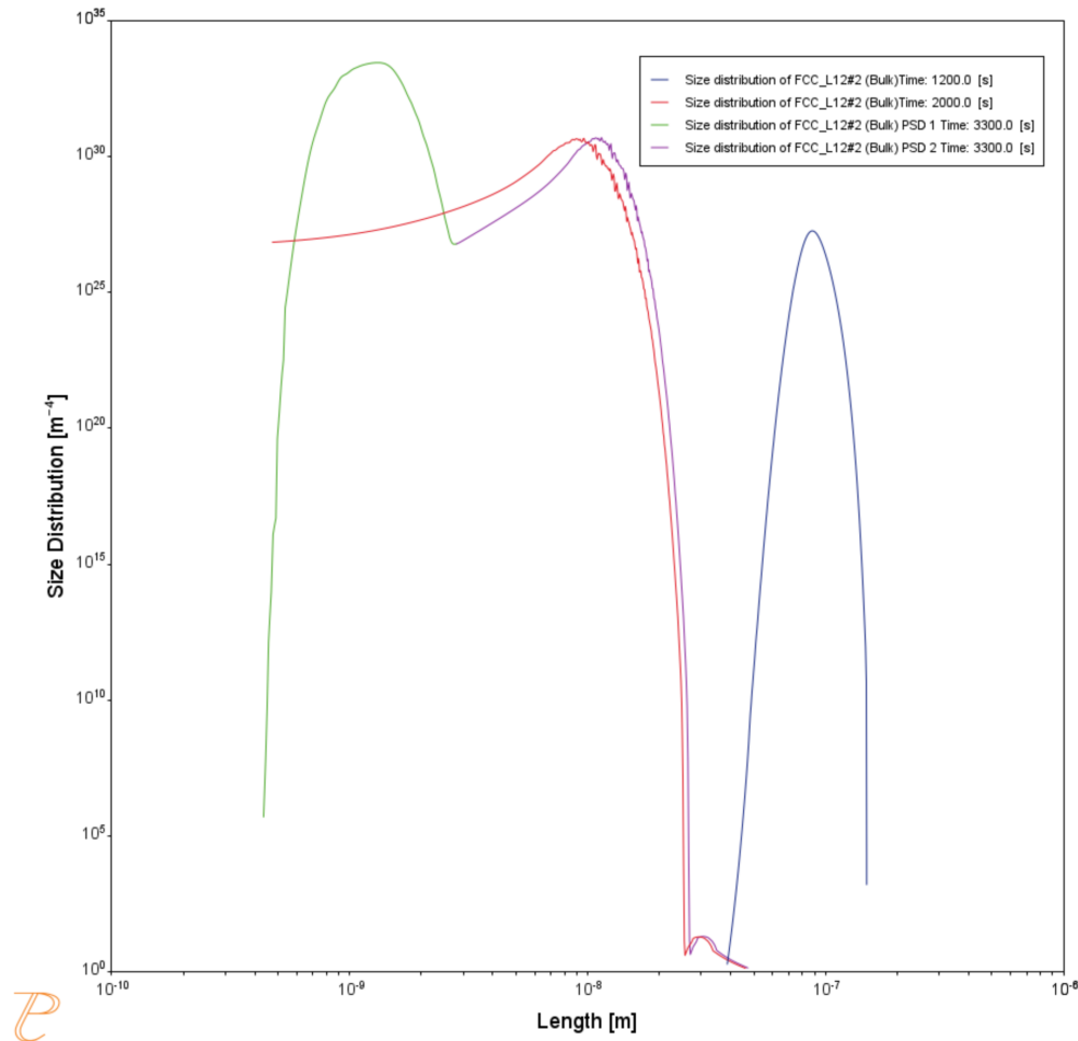
Figure 25: Preexisting Size Distribution (PSD) Ni-10Al-10Cr.
