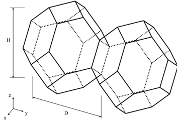
Figure 7: An example of tetrakaidecahedron approximation of grains.
