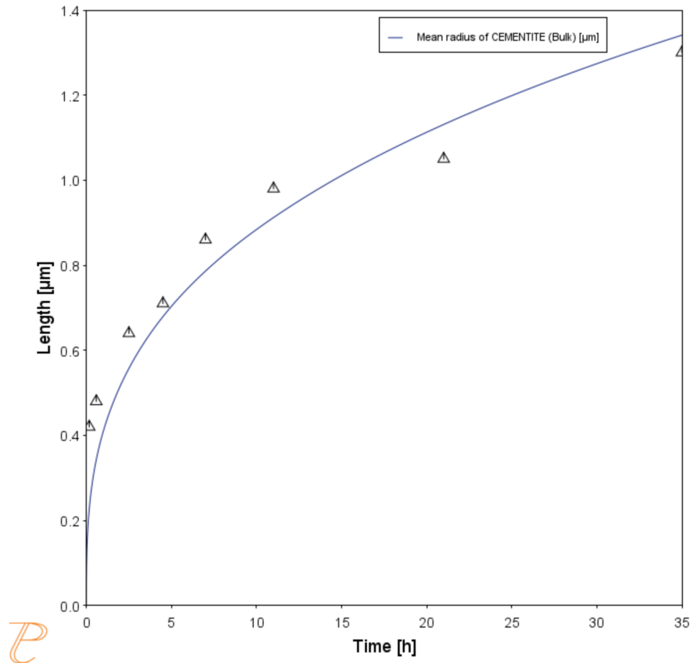
Figure 42: Result comparing the cementite mean radius to experimental data from [1975Hel].
