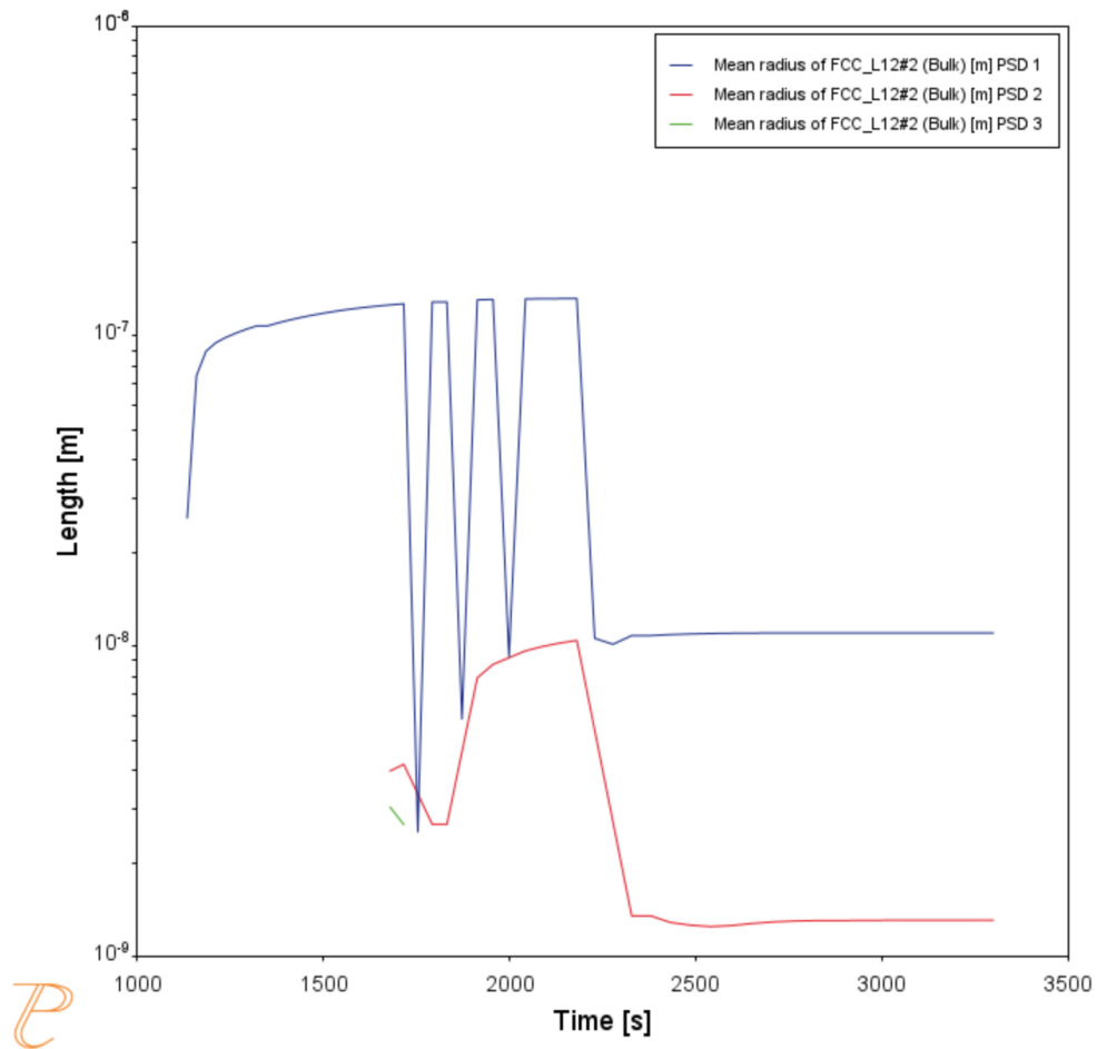
Figure 23: Mean radius Ni-10Al-10CR.
