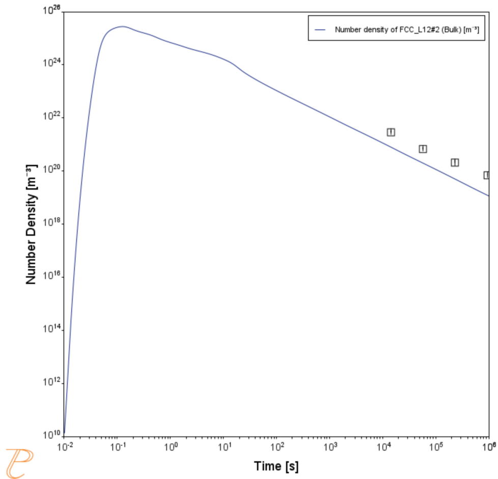
Figure 20: The results of an isothermal calculation to plot the number density of the cementite phase.
