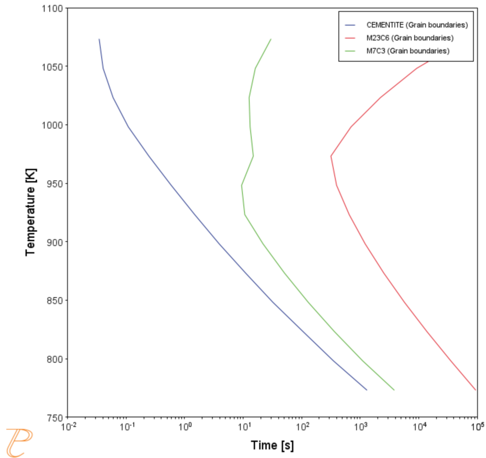
Figure 17: The Precipitation Calculator is used to do a TTT (Time-Temperature-Transformation) diagram calculation of the three phases (cementite, M23C6 and M7C3) at the grain boundaries.
