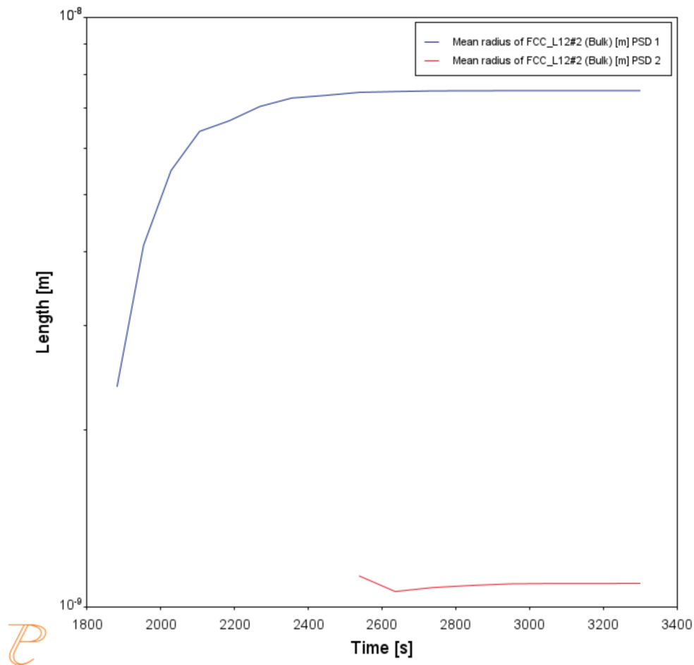
Figure 22: Mean radius Ni-8Al-8Cr.
