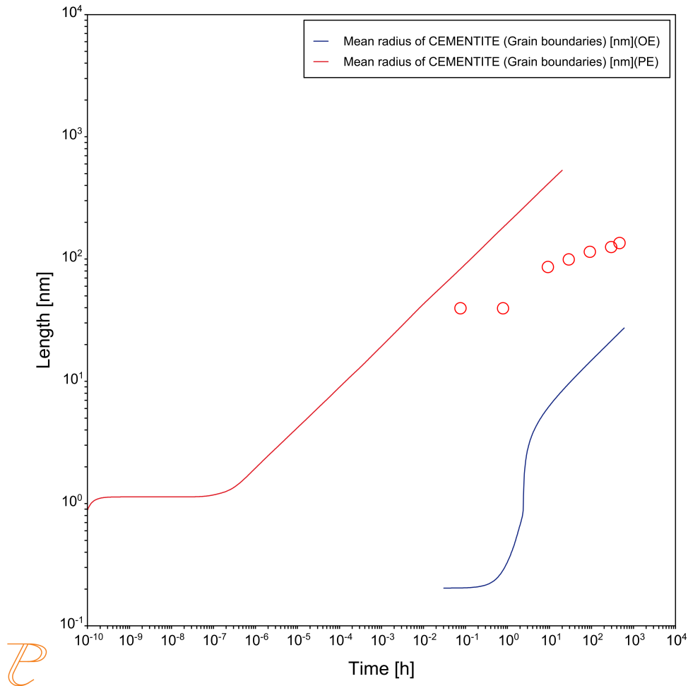
Figure 41: Comparing results from Para-eq (PE) and Simplified (OE) growth models.
