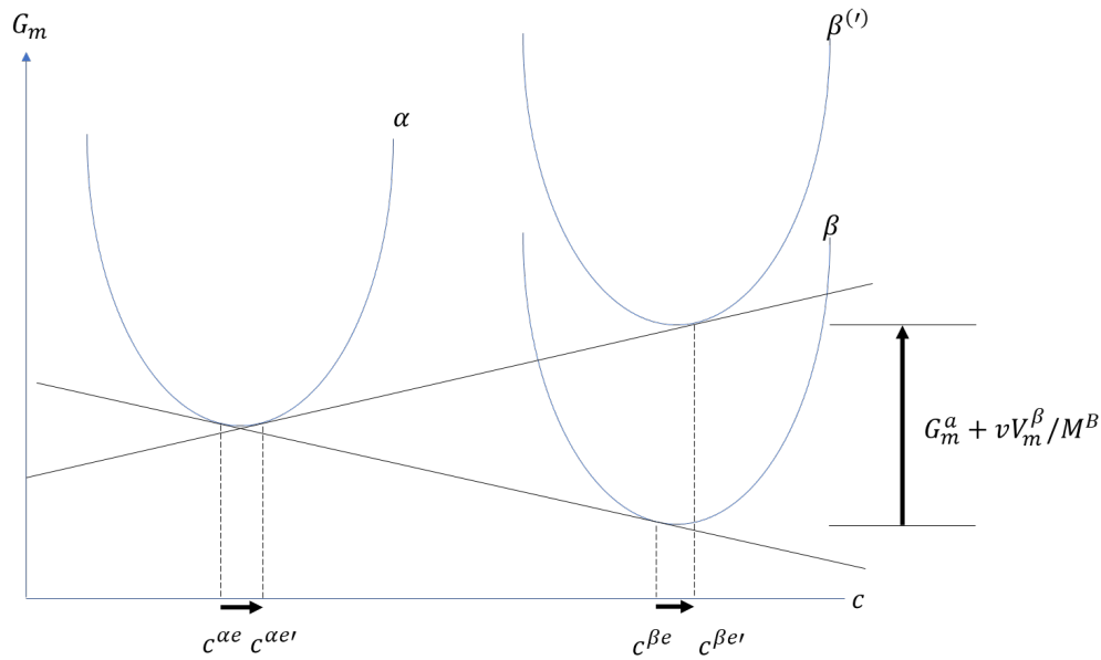
Figure 8: Effects of “Phase energy addition” G_m^a and “Phase boundary mobility” M^B .
