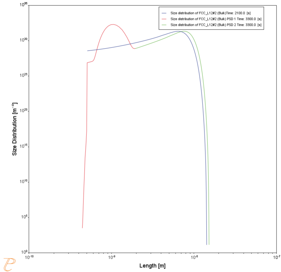
Figure 24: Preexisting Size Distribution (PSD) Ni-8Al-8Cr.
