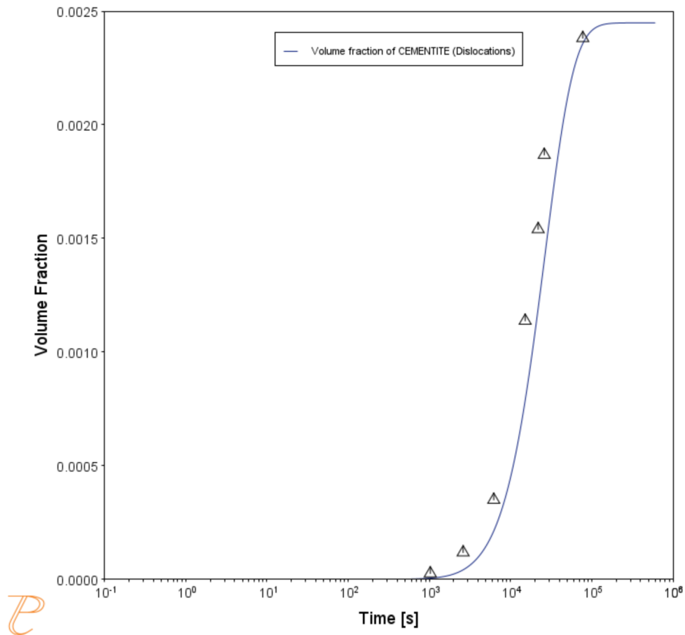
Figure 18: Volume fraction of the cementite phase.
