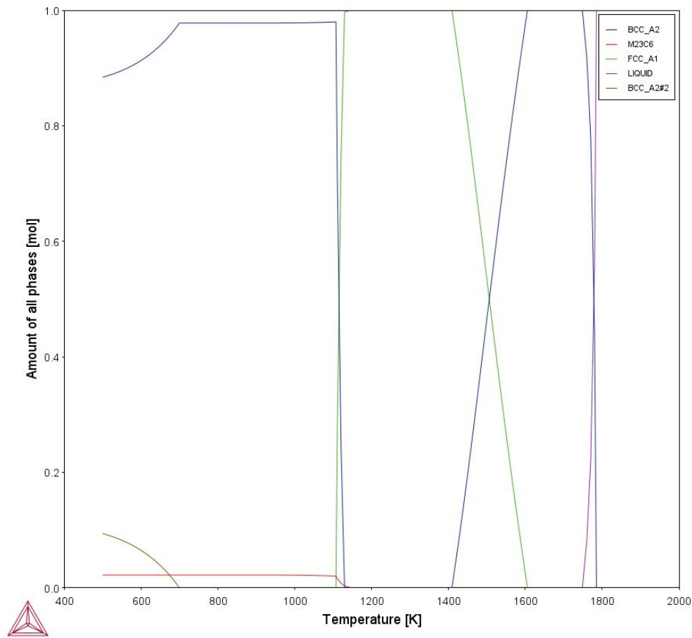
Figure 16: The Equilibrium Calculator is used to show how the phases change with temperature.
