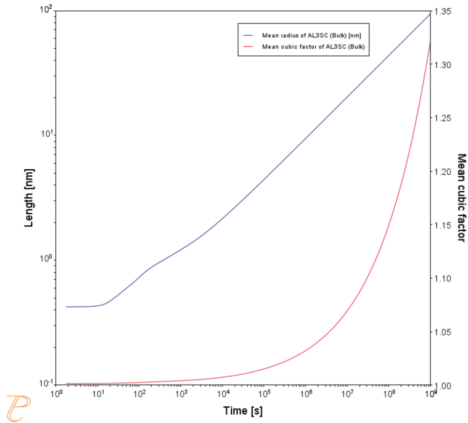
Figure 34: Mean Radius and Cubic Factor
