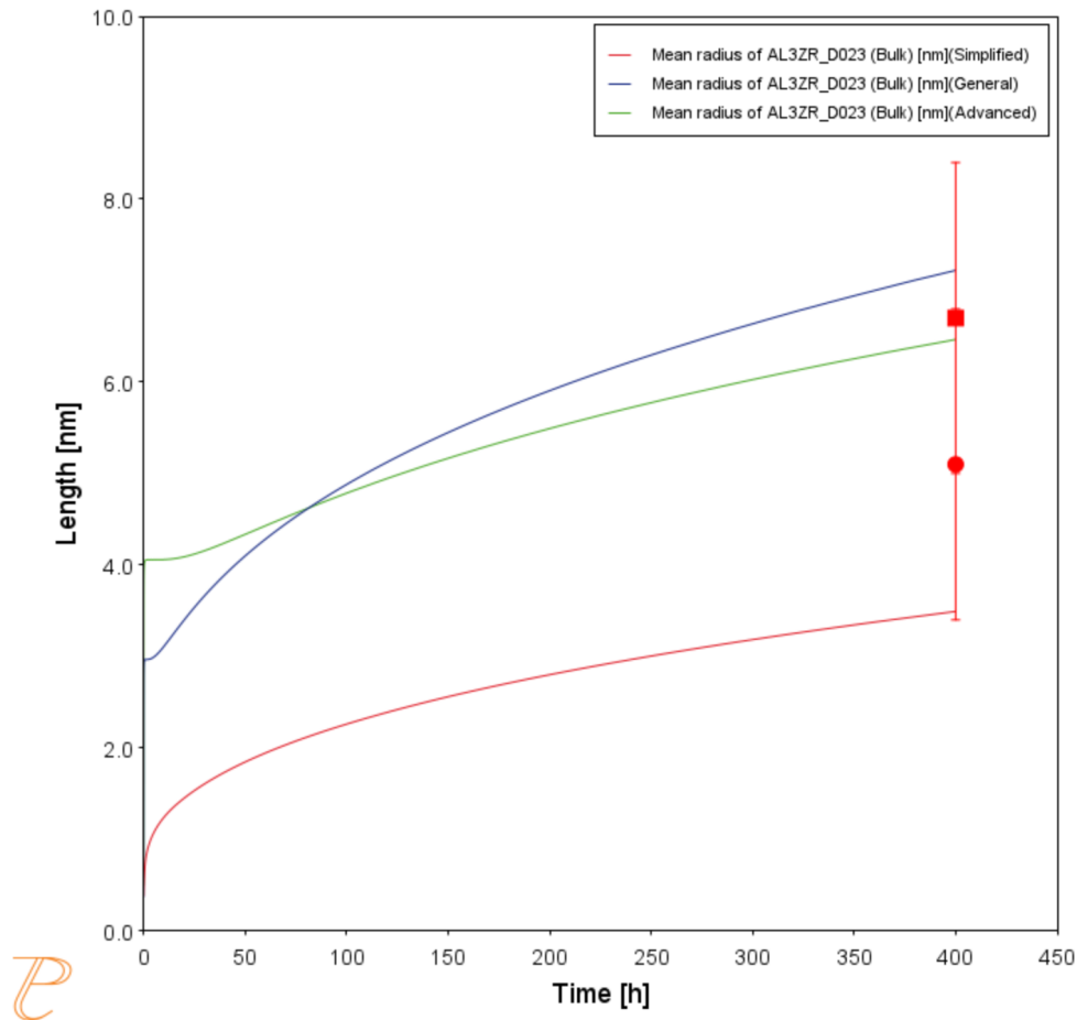
Figure 40: Result comparing the mean radius of the spheres for each AL3ZR_D023 precipitate phase calculated for each type of growth rate model.
