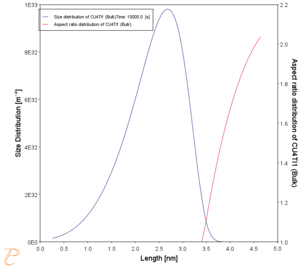
Figure 30: PSD and ASD.
