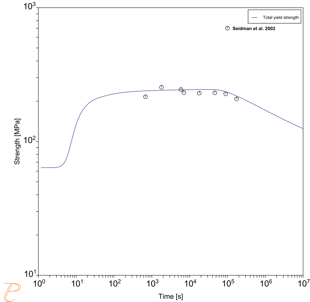
Figure 13: The total yield strength of the Al_3Sc precipitate as a function of time compared to experimental data from Seidman et al. [2002Sei].
