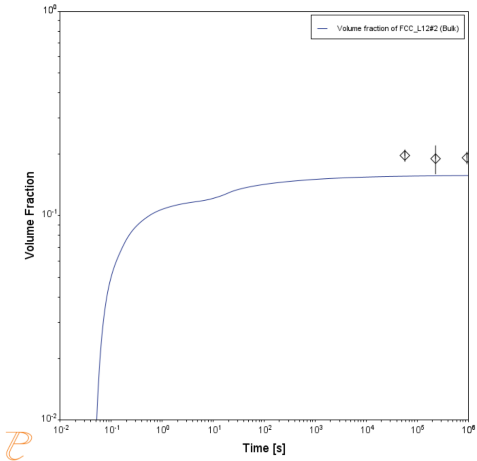
Figure 19: The results of an isothermal calculation to plot the volume fraction of the cementite phase.
