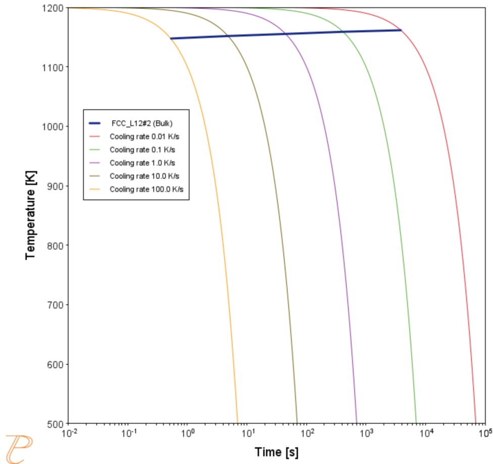
Figure 26: In this plot, the blue horizontal line shows the time it takes for \gamma' to transform at each of the cooling rates according to the stop criteria, which is set as 1e-4 volume fraction. The cooling rates are represented by the multicoloured curved lines.
