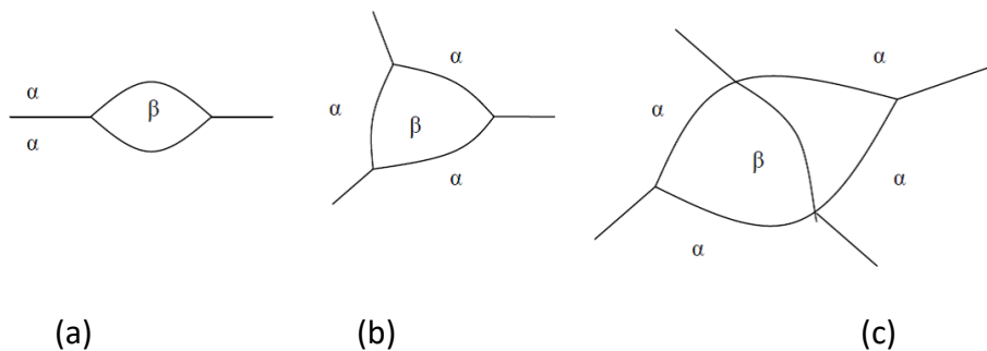
Figure 5: Non-spherical particles ( \beta ) that precipitate at grain boundaries of matrix phase( \alpha ) (a) grain boundary (two-grain junction) (b) grain edge (three-grain junction) (c) grain corners (four-grain junction). Images from [2004Zan].
