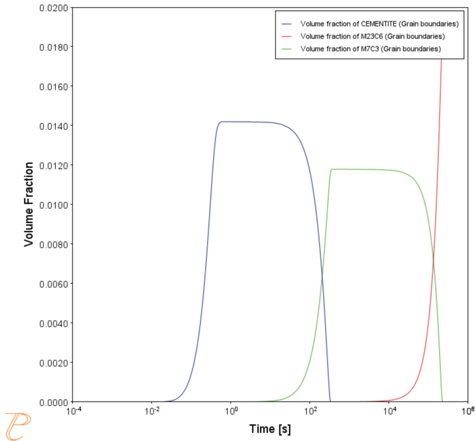
Figure 15: The Precipitation Calculator is used to do an isothermal calculation of the three phases (cementite, M23C6, and M7C3) where cementite and M7C3 are metastable phases.
