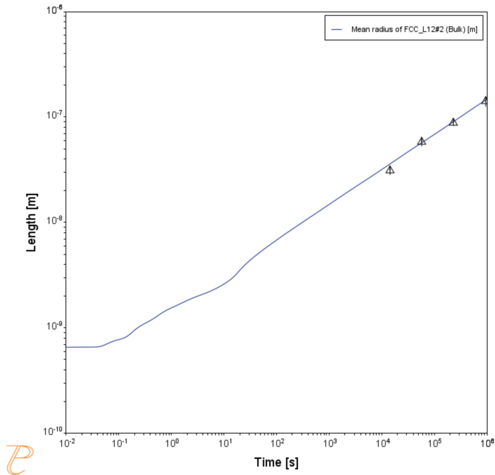
Figure 21: The results of an isothermal calculation to plot the mean radius of the cementite phase.
