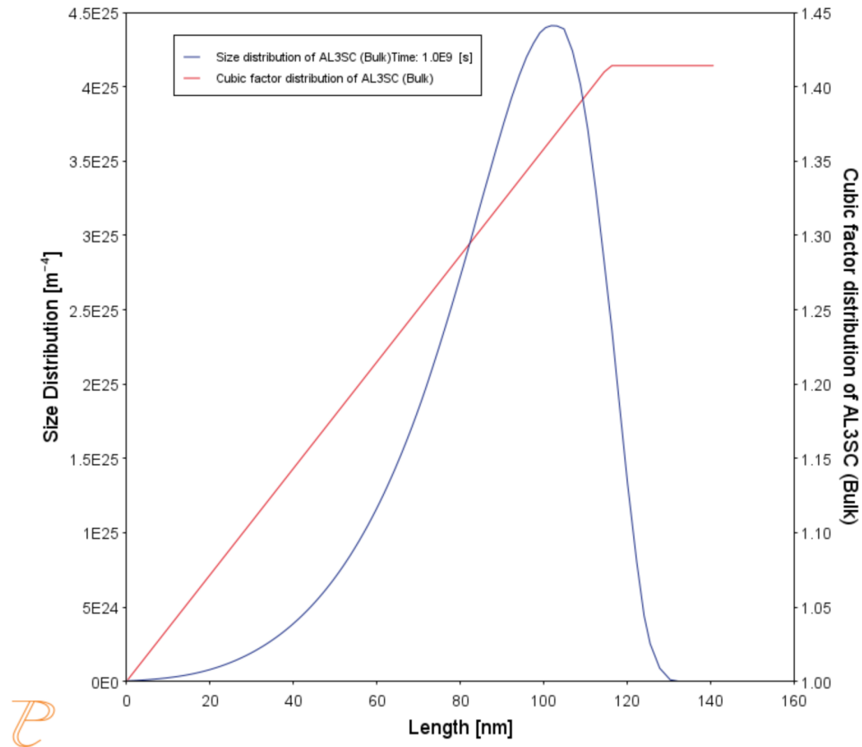
Figure 35: Particle size distribution (PSD) and cubic factor.
