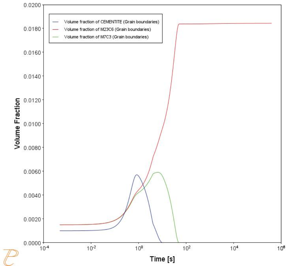
Figure 37: Volume fraction with initial particle size distribution (PSD).
