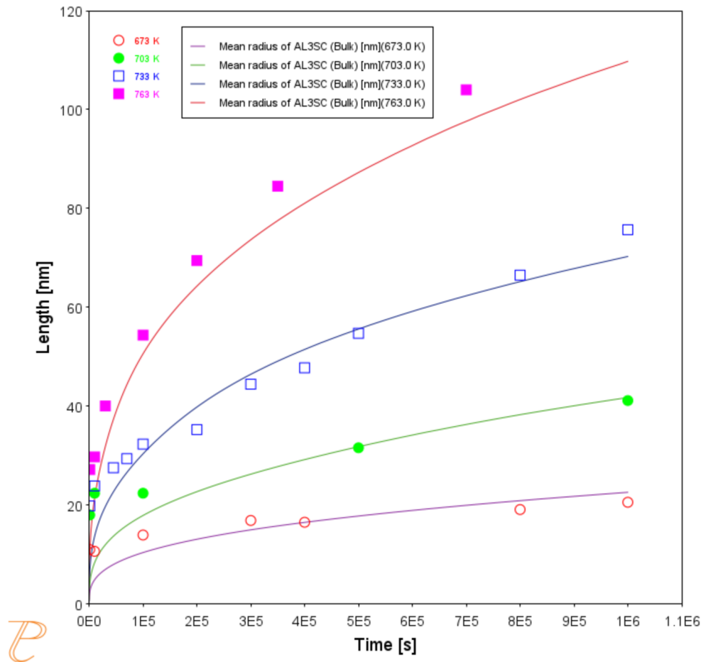
Figure 39: The results of an isothermal calculation to examine the mean radius of an Al-0.12Sc system with experimental data from [2004Iwa].
