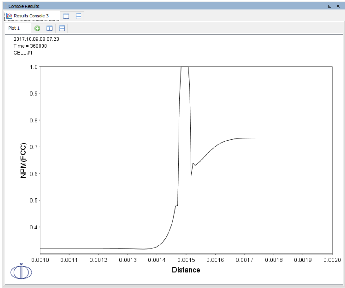
Output from the multiphase_example showing the mole fraction fcc phase as a function of distance at the end of the heat treatment.
