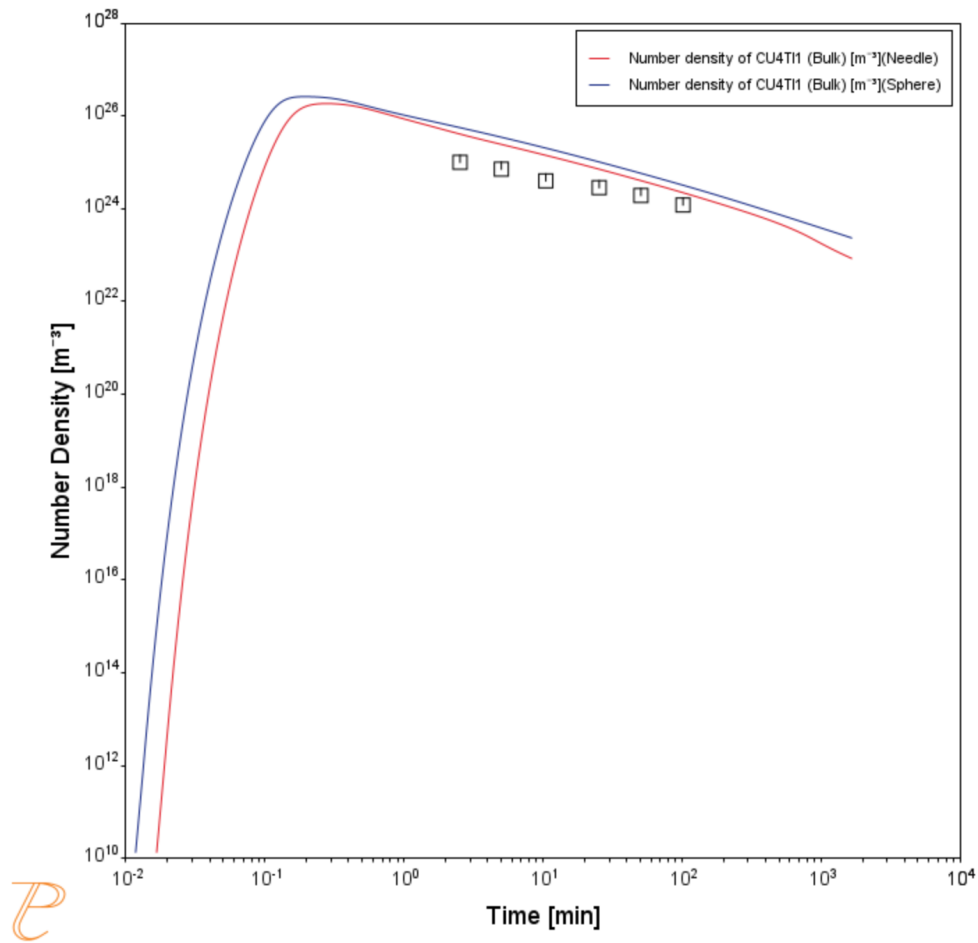
Figure 30: Number Density.
