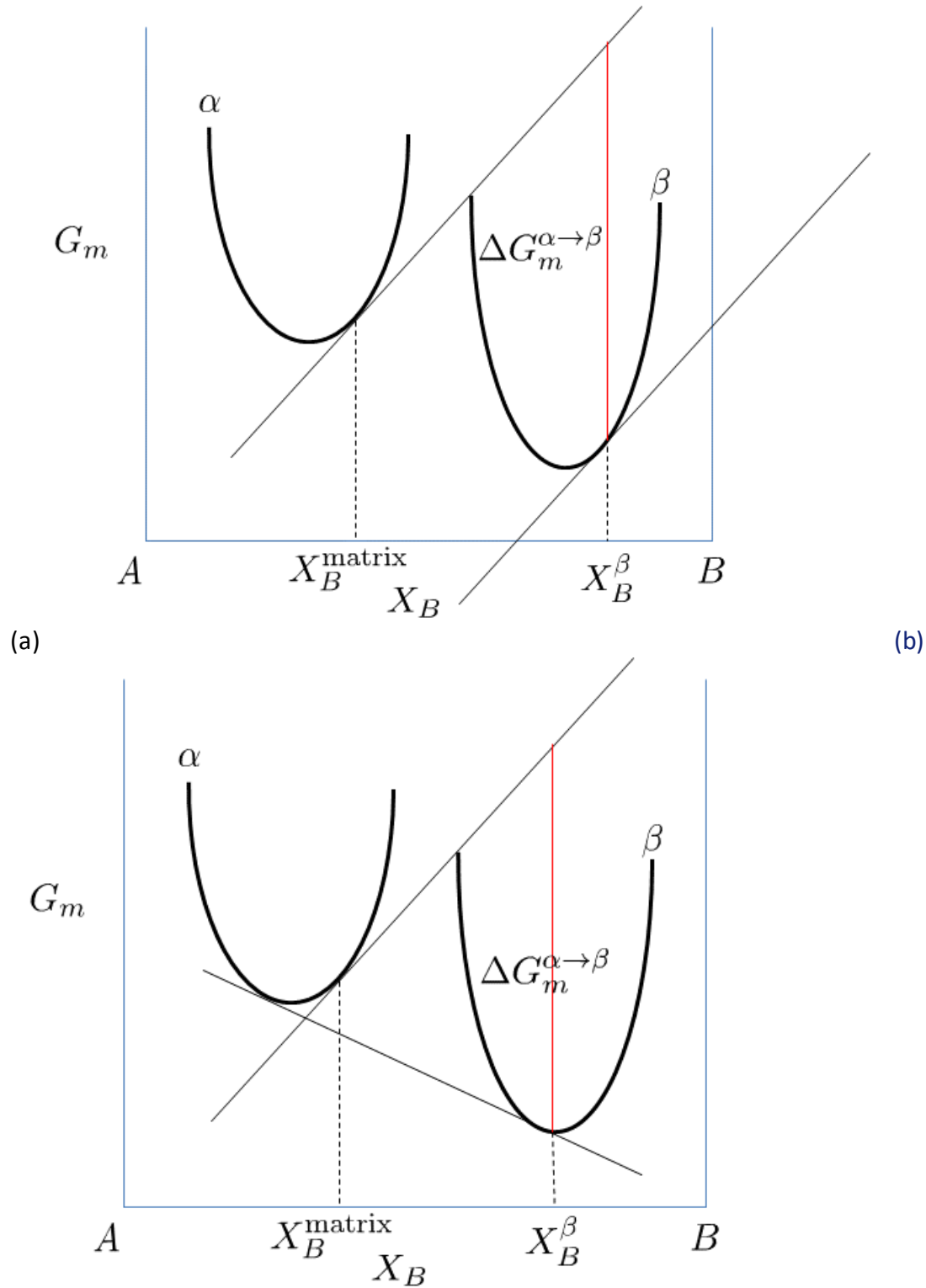
Figure 1: Methods to calculate the nucleation driving force \Delta G_m^{\alpha \rightarrow \beta} and the critical composition X_i^\beta . The left-hand side figure (a) is a standard calculation and the right-hand side (b) an approximate calculation.
