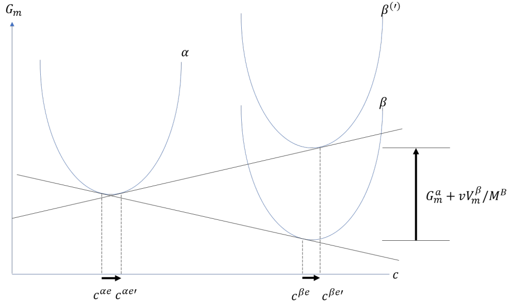
Figure 1: Effects of “Phase energy addition” G_m^a and “Phase boundary mobility” M^B .
